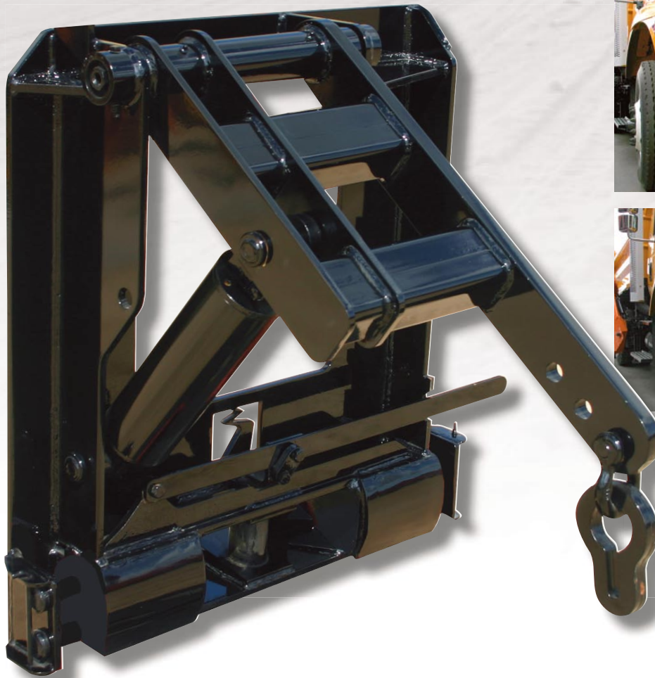
Fig. 1: QX shown in the lowered or down position.
