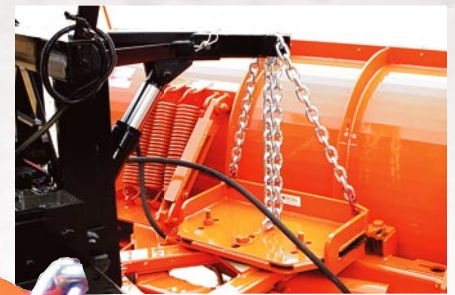
Fig. 1: Can be set in any of 3 sets of holes enabling different degrees of leveling capability, increasing the workability with different types of hitch/lift arm combinations
